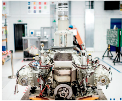
Main Gearbox
