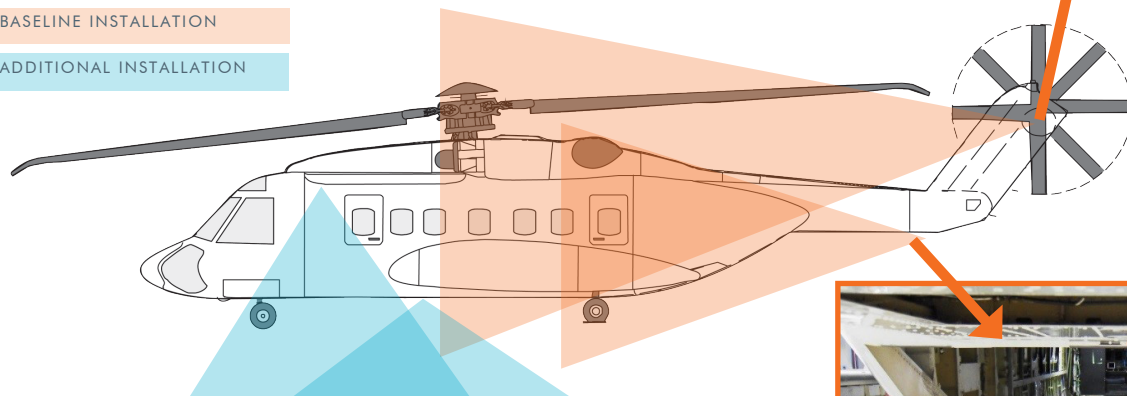
S-92 WITH CAMERA INSTALLATION FIELD OF VISION
