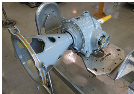
TAIL GEARBOX IN THE WORKSHOP
